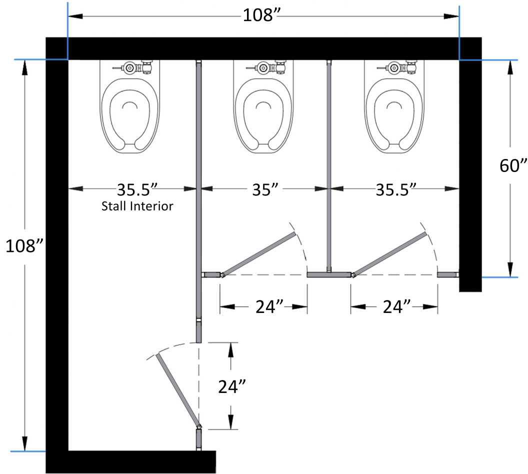
Bathroom Partitions - 3 Stall Alcove Left Hand SKU: AL3L Standard Dimensions
